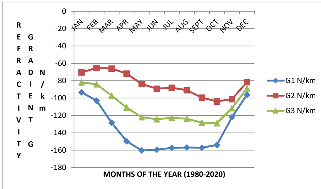
Figure 2: Yearly Vertical Radio Refractivity Gradient Monthly Average Variations across Abuja (1980-2020).
