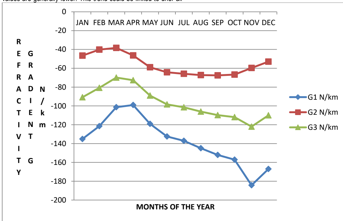
Figure. 4 shows annual average monthly variations in the vertical radio refractivity gradient above Makurdi (1980-2020).
