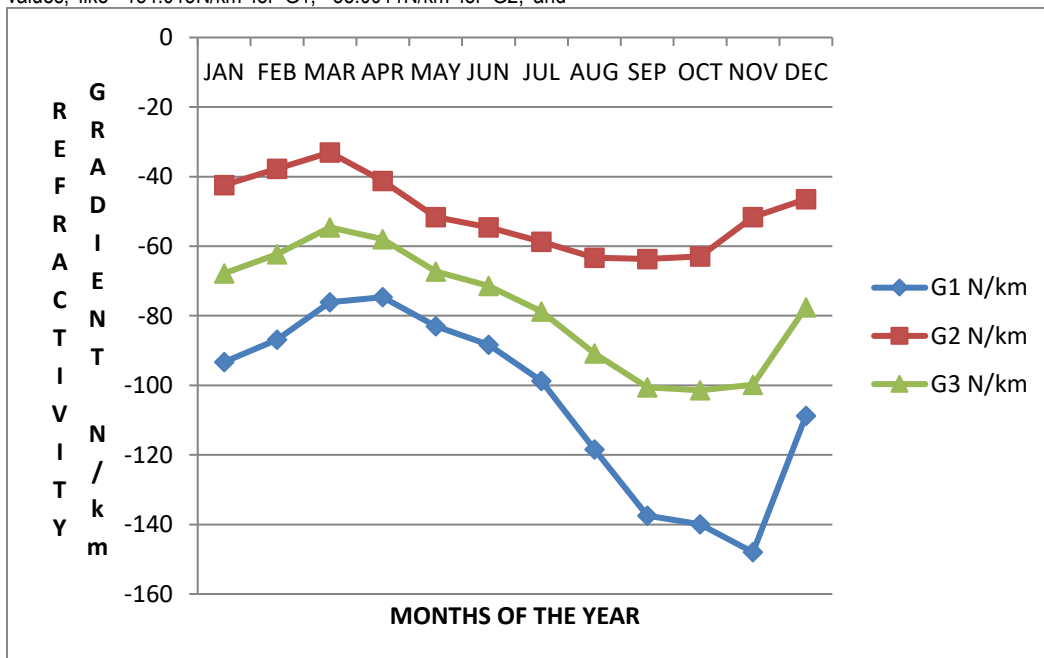
Figure 3: Monthly Average Variations of Vertical Radio Refractivity Gradient over Jos in the year (1980-2020).
